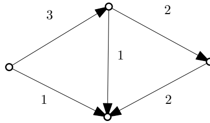
Figure 1: An example of a \mathbb{Z}_4 -flow.
