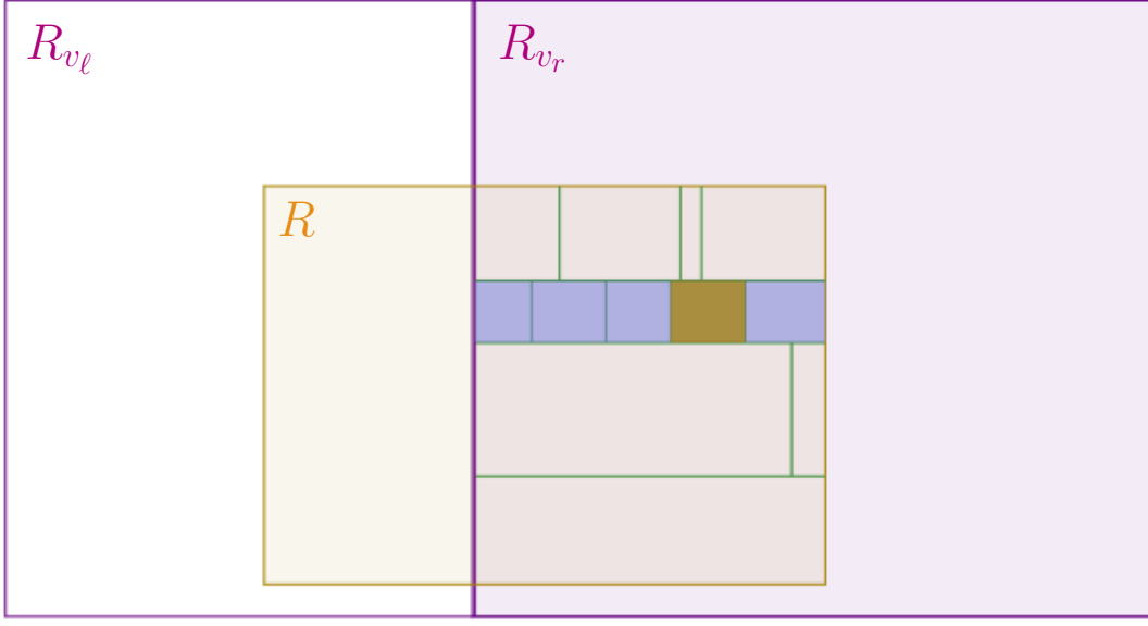
Figure 3: One iteration of Simulation Protocol . We perform Rectangle Partition (green lines) on the larger half of R after moving from v to its child (shaded in purple), use Lemma 5.5 to identify a part j (shaded in blue), and then query I_j and set R to X^j \times Y^{j,\beta} for the result z[I_j] = \beta (shaded in brown).
