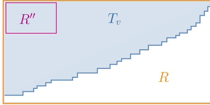
Figure 3: One iteration in Decision-tree . R is split by the triangle T_v , with R' (not pictured) being the largest rectangle either contained in T_v or disjoint from it. After using Round Lemma and querying the appropriate bits we go into the next round by updating R \leftarrow R'' .
