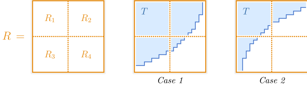
Figure 2: Simple fact: for every rectangle R and triangle T there is a subrectangle R' \subseteq R with |R'| \geq |R|/4 that is either contained in T or disjoint from it. Namely, after permuting the rows and columns of R according to T 's orderings, take either the first quadrant R_1 or the fourth R_4 .
