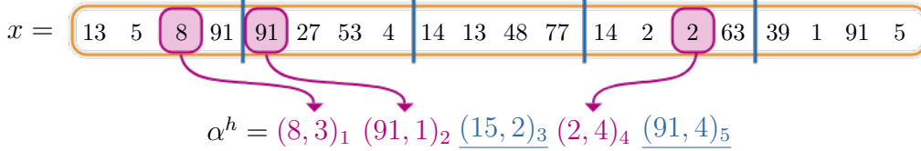
Figure 5: Example of sampling \alpha^h for d^3 = 5 megacoordinates of size mN/d^3 = 4 . Here (I_j, \alpha_j) for I_j = \{3, 5, 15\} and \alpha_j = \{(8)_3, (91)_5, (2)_{15}\} is sampled. (8)_3 goes to (8, 3) in the first coordinate, (91)_5 goes to (91, 1) in the second coordinate, and (2)_{15} goes to (2, 4) in the fourth coordinate. For the third and fifth coordinate a pair in [m] \times [5] is chosen uniformly, choosing (15, 2) for the third and (91, 4) for the fifth.
