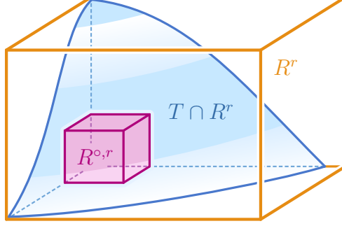
Figure 1: Structured case of Simplex Lemma . The simplex T is partitioned as T = \bigsqcup_r T \cap R^r where each structured part is sandwiched between two \rho^r -structured boxes, R^{o,r} \subseteq T \cap R^r \subseteq R^r .
