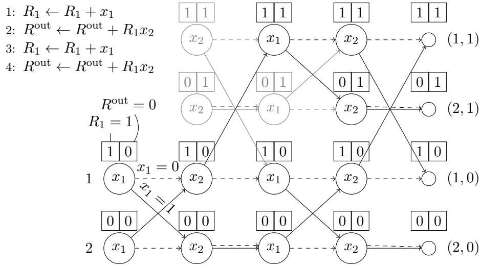
Figure 2: A transparent register program computing \text{AND}(x_1, x_2) , and its realization as a 2-catalytic branching program using Observation 1. Each node is annotated (above, in boxes) with the register values it stores, and each non-sink node is labelled (inside the circle) with the input to be read. Dashed lines are transitions taken when that input is zero, and solid lines are taken when the input is one. Finally, the source nodes are assigned the numbers 1 and 2 (since m = 2 ), and the sink nodes are assigned pairs of numbers, so that like in the more abstract Figure 1, a computation starting at source node v will end at end at sink node (v, f(x)) . Note that nodes/edges that appear in gray are unreachable from the start states and thus would not appear in the final branching program; they appear only for reference as to how the register program translates to a branching program.
