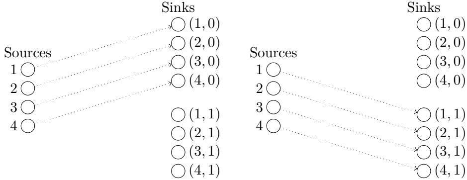
Figure 1: The computation of an m -catalytic branching program starting at source node i ends at sink node (i, 0) if f(x) = 0 (left) or (i, 1) if f(x) = 1 (right). In these diagrams, m = 4 .
