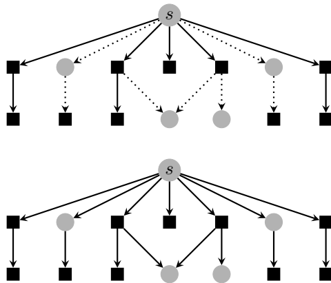
FIG. 4. An example of extended neighborhood of Steiner vertex s . The set N_{Ext}^0(s) is depicted on the top using full arcs, while the vertices connected by dotted arcs are not a part of this set. The set N_{Ext}^1(s) is depicted on the bottom using full arcs.
