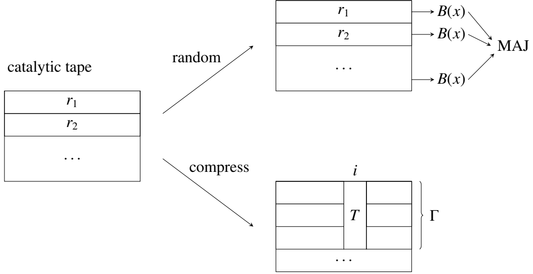
Fig.: compress-or-random argument
