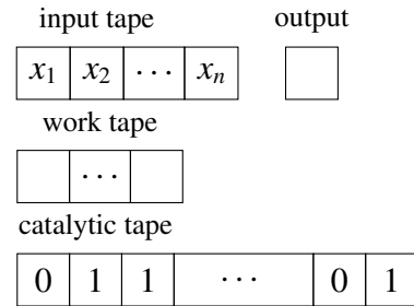
Fig.: catalytic Turing Machine
