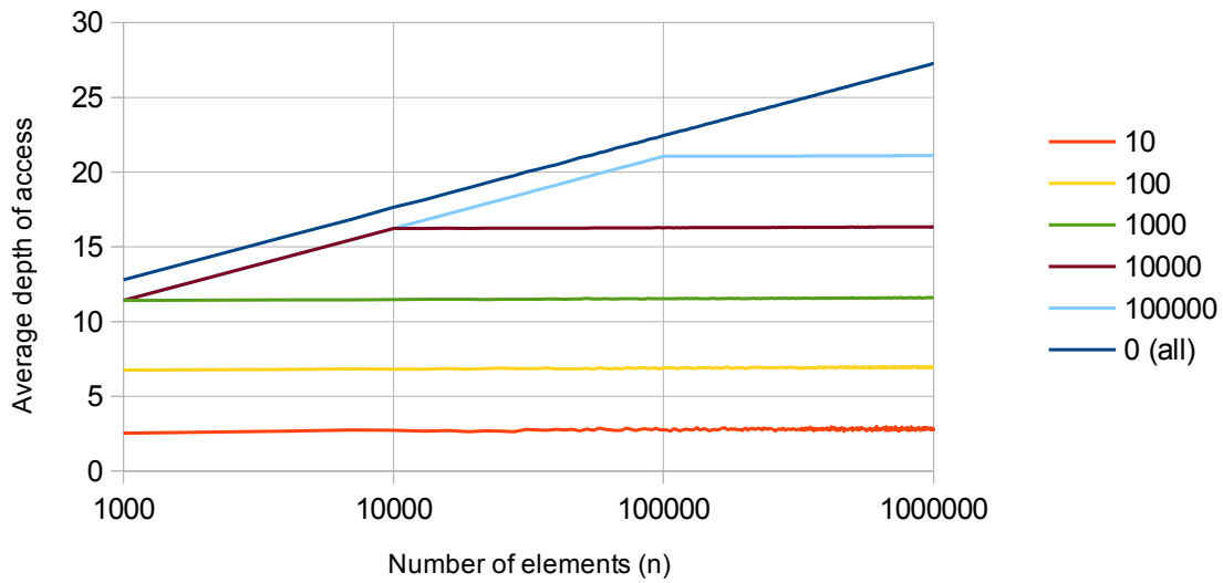
Splay tree performance: accessing subsets of various sizes (N)
